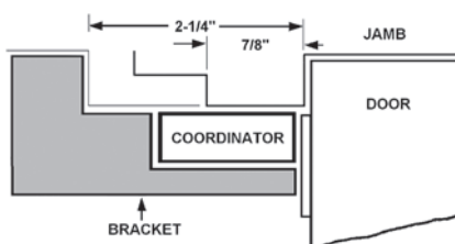
PCORMB434 Mounting Bracket (1 step) Jamb Depth 4-3/4" Min. 5/8" Stop Height - For Stop over 2-1/4" (sold as pair)
